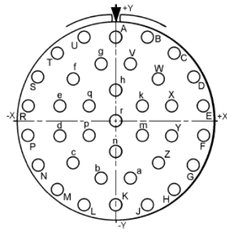
Contact Layout
