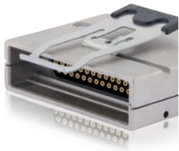
microComp® Quick latch Removable contacts Up to 175°C High vibration withstanding
